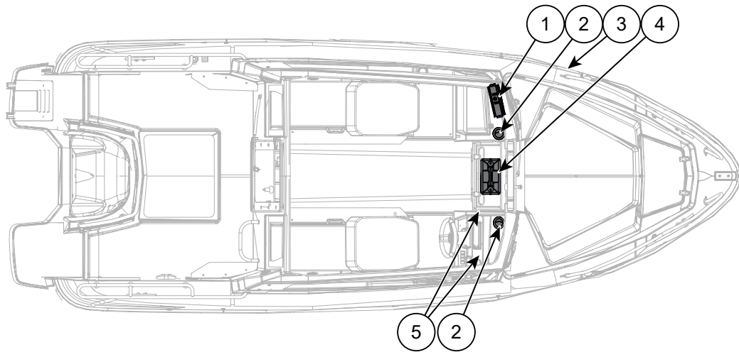
Figur 6.2 Cross 60 Cabin varmeapparat
