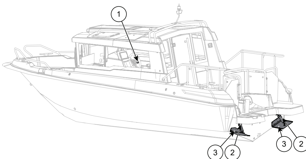
Figur 5.5 Cross 60 Cabin trimsystem
