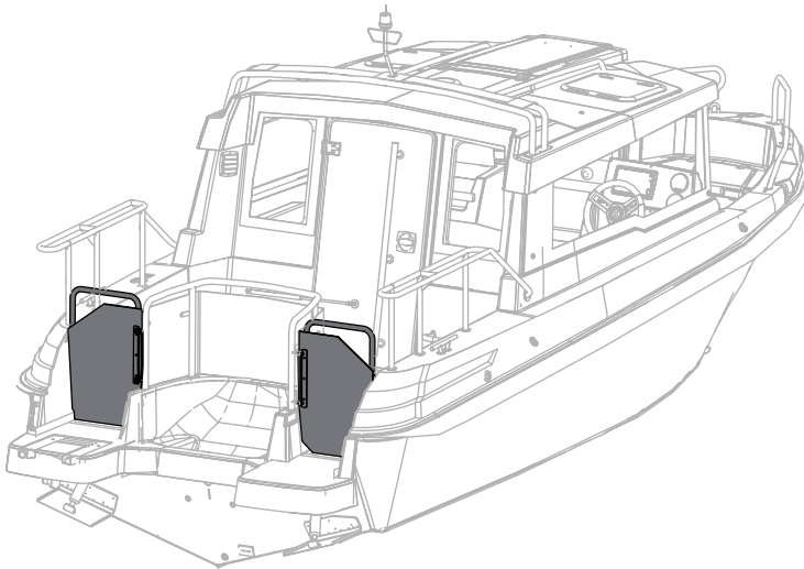
Figur 4.2 Cross 60 Cabin ombordstigningsporter
